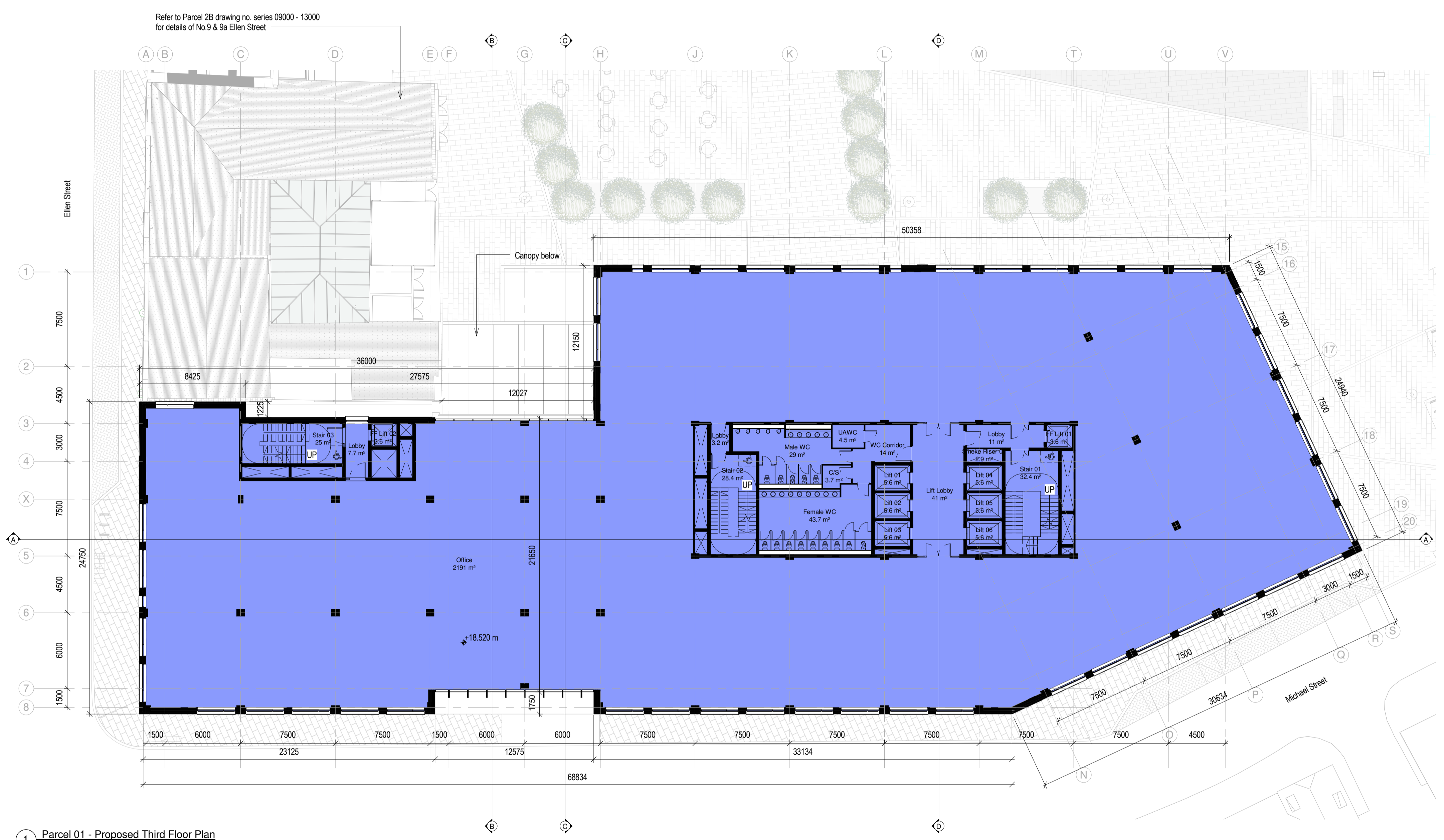
1 Parcel 01 - Proposed Third Floor Plan 1:200
